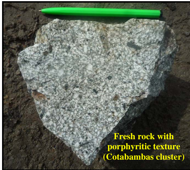
Foto N° 5.5.- Porphyritic texture of the fresh rock of the Cotabambas cluster.
