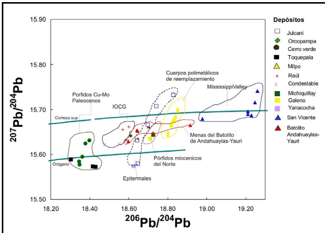
Figure 5.5: Comparison of Pb isotopic ratios of some samples of ore from Andahuaylas - Yauri Batholith with other peruvian deposits. ^{207}\text{Pb}/^{204}\text{Pb} vs ^{206}\text{Pb}/^{204}\text{Pb} diagram showing Pb isotopic comparison of different deposits.
