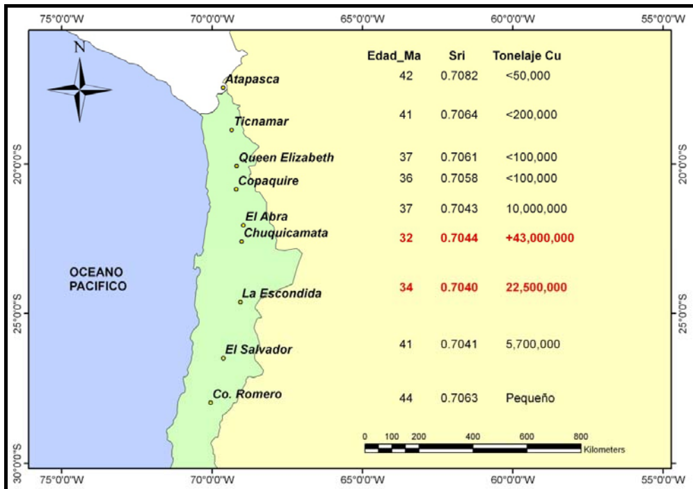
Figure 5.6: Comparison of age, initial isotopic ratios of Sr 87 /Sr 86 and tonnages of different Porphyry deposits of Chile. (Courtesy of F. Munizaga in Tassinari, 2006)
