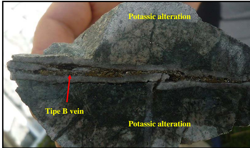
Photo N° 5.1.- Type B vein, with a central suture of sulfides (pyrite and chalcopyrite, notice the potassic alteration).
