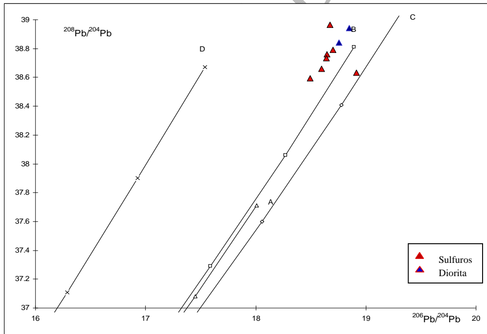
Figure 5.3: Isotope compositions Diagram of ^{208}\text{Pb}/^{204}\text{Pb} vs ^{206}\text{Pb}/^{204}\text{Pb} for samples of ore and fresh rock at NW area of Andahuaylas-Yauri Batholith. It was used as reference curves of Pb isotopic evolution established for Plumbotectónico-Toriogénico model of Zartman & Doe (1981).
