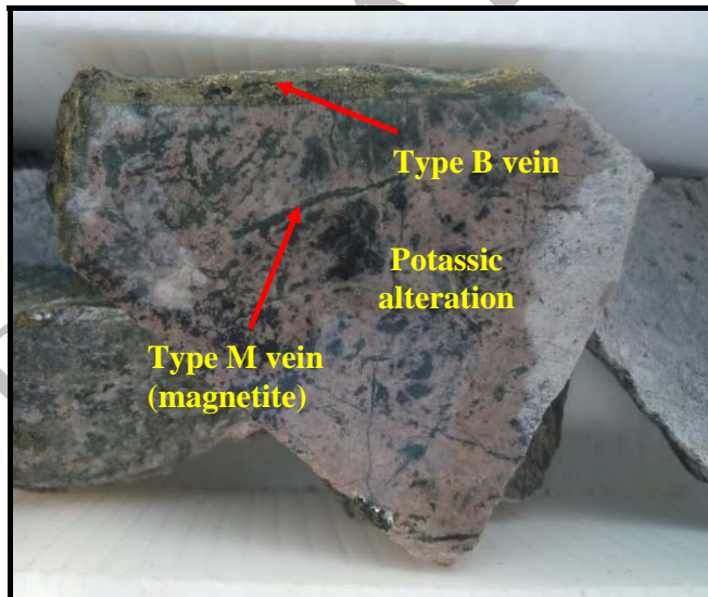
Photo N° 5.4.- Type B and M veins with potassic alteration of the main porphyry
