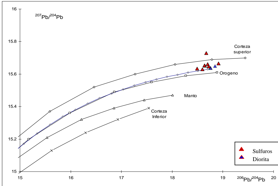
Figure 5.2: Isotope compositions diagram of ^{207}\text{Pb}/^{204}\text{Pb} vs ^{206}\text{Pb}/^{204}\text{Pb} for samples of ore and fresh rock at NW area of Andahuaylas-Yauri Batholith. It was used as reference curves of Pb isotopic evolution established for the Plumbotectónico-Uranogénico model of Zartman & Doe (1981).
