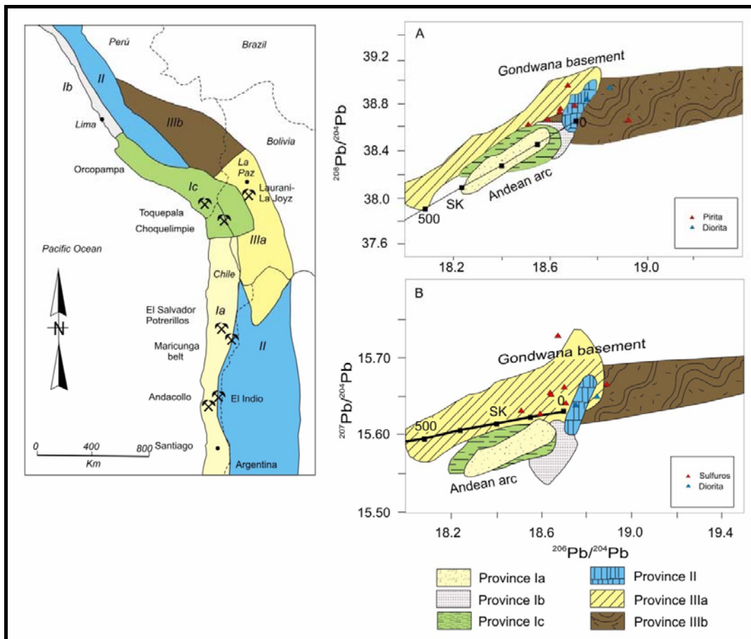
Figure 5.4: Map Pb isotopic provinces of the Central Andes and Thorogénico diagrams (A) and Uranogénico (B) containing samples of ore and rock in the NW sector of the Andahuaylas – Yauri Batholith (Modified from Macfarlane et al., 1990 by Tosdal et al., 1999).
