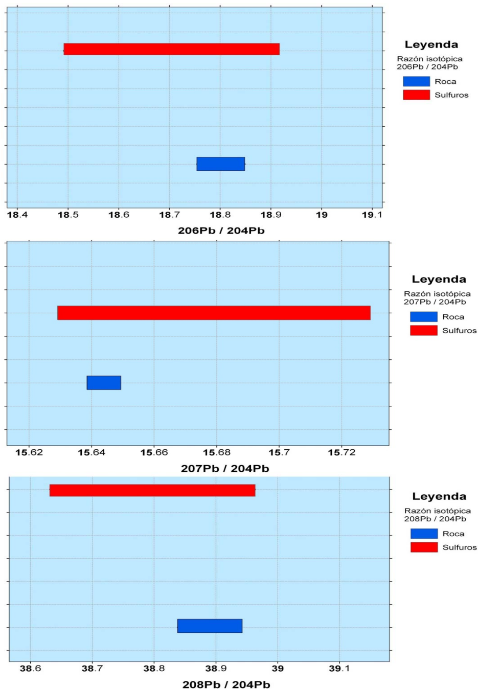
Figure 5.1: Comparison of ranges of isotopic ratios of ^{206}\text{Pb}/^{204}\text{Pb} , ^{207}\text{Pb}/^{204}\text{Pb} and ^{208}\text{Pb}/^{204}\text{Pb} of mineralization and host rock.
