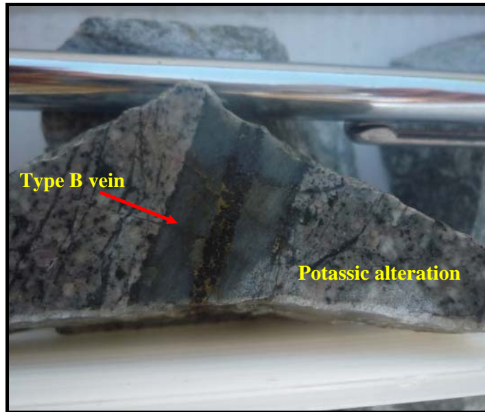
Photo N° 5.3.- Type B vein within potassic alteration, notice the central suture of pyrite and chalcopyrite (Cotabambas cluster)
